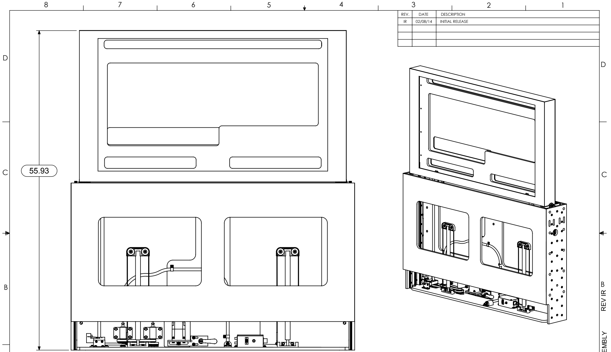
DETAIL -1 (DEPLOYED POSITION)
